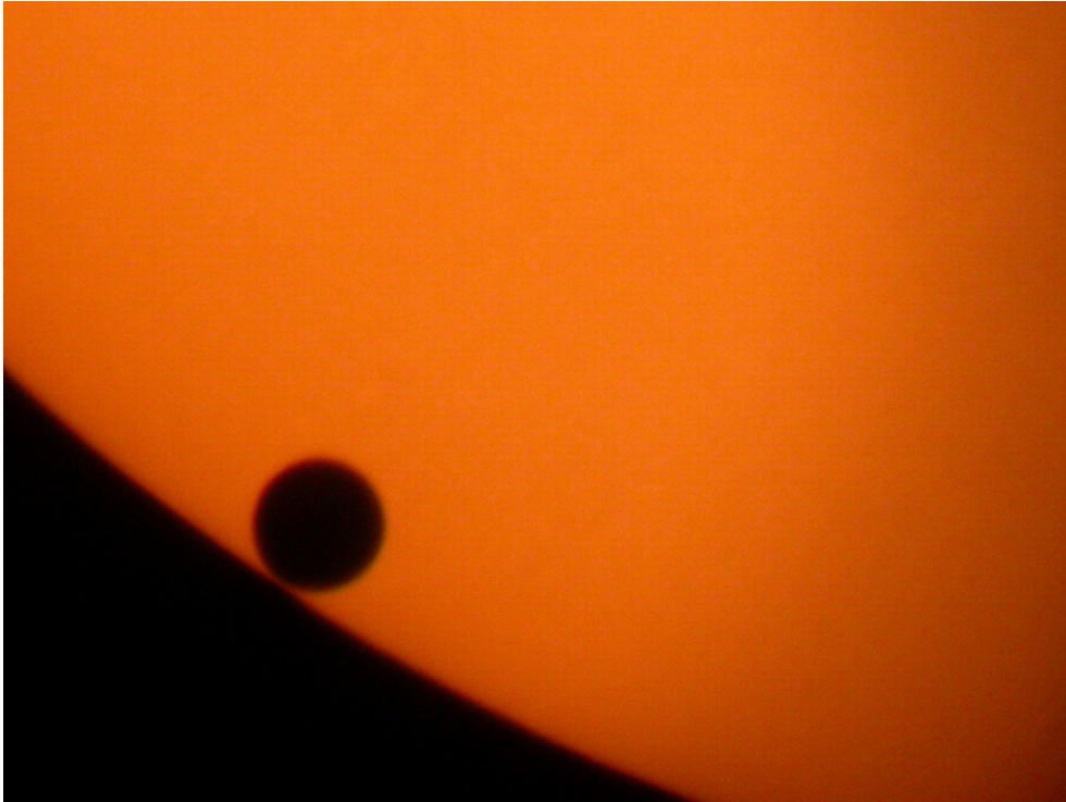
Transit of Venus in front of the Sun. Author: O. González
